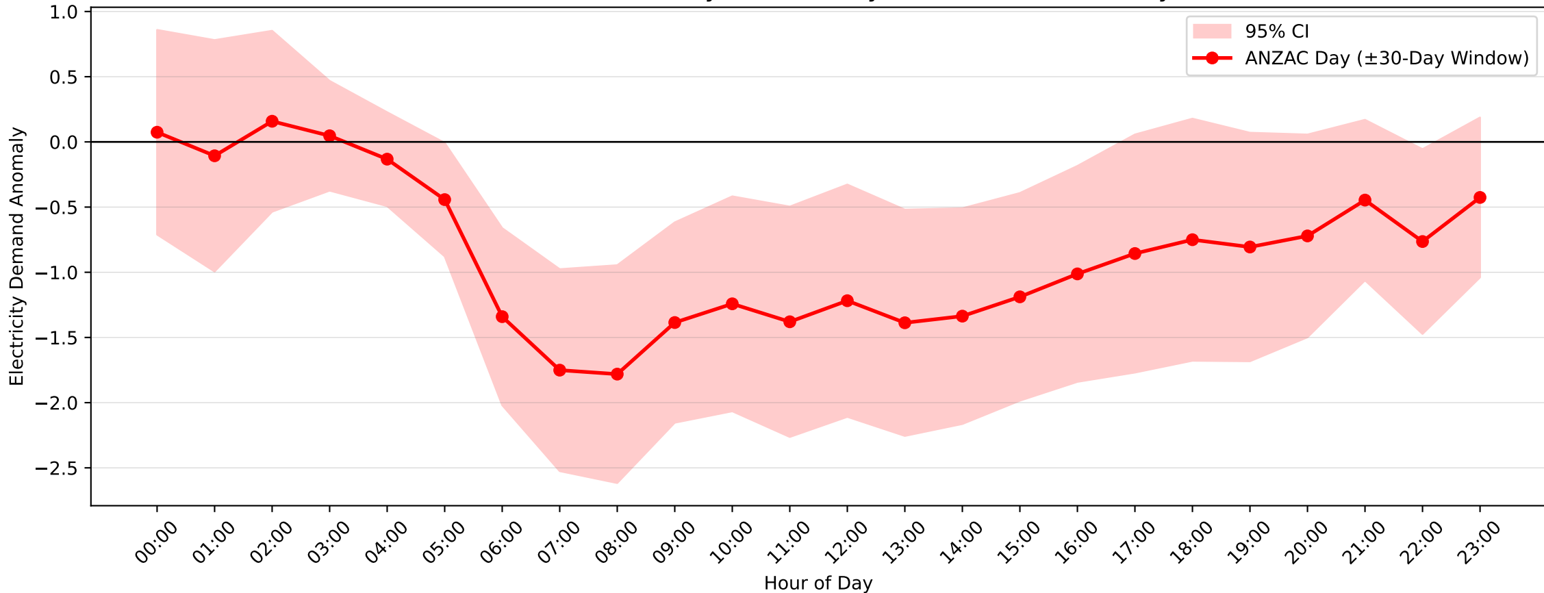
Gateshead Demand Anomaly: ANZAC Day (2004–2017, \pm 30 -Day Window)
